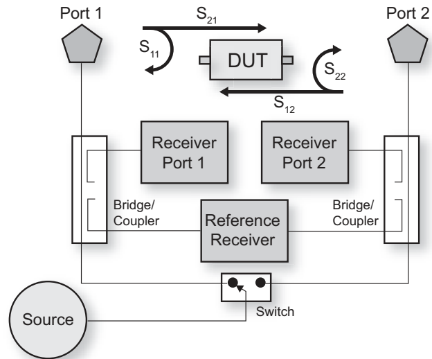
The above illustration is a simplified block diagram of VNA Master's architecture.
